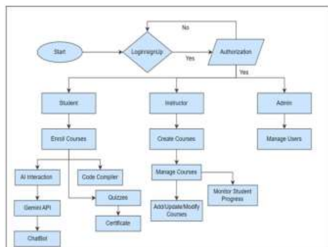
Figure 2 - Flowchart
