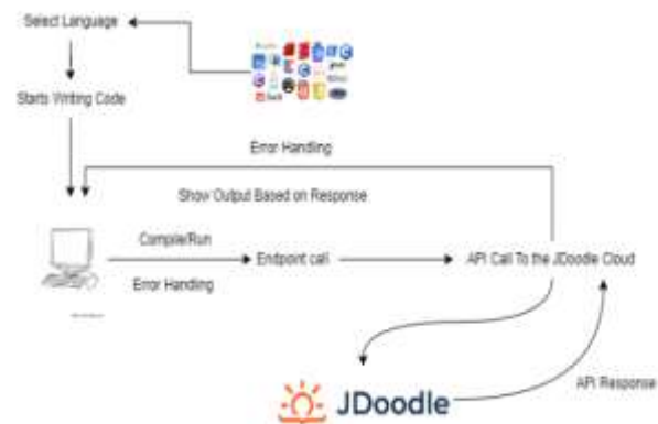
Figure 1 - JDoodle API Workflow
